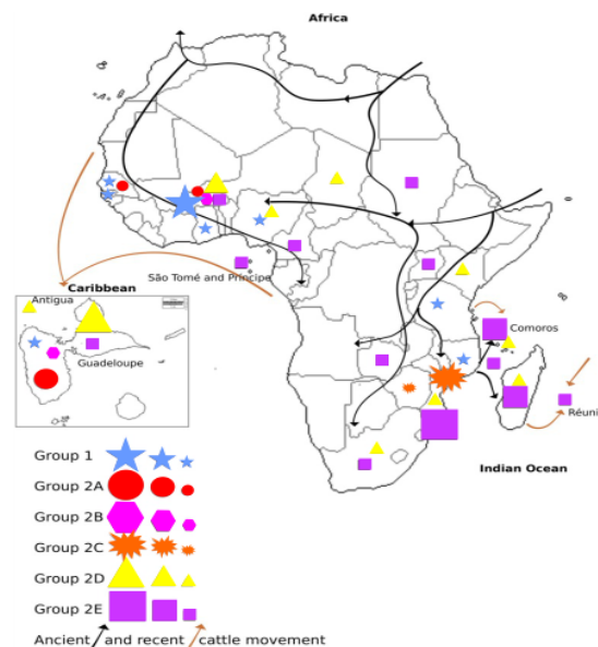
Figure 3: Distribution of E. ruminantium genetic groups and subgroups 1, 2A, 2B, 2C, 2D, and 2E in each sampled country within Africa, Caribbean, and Indian Ocean Islands. Groups are coded by symbols according to the legend. Symbol size corresponds to sampling size defined by the following sample threshold: >15 samples (big symbol), < 15 samples (medium symbol), and < 5 samples (small symbol). Recent (< 400 years ago; brown arrows) and ancient (>400 years ago; black arrows) movement of cattle is represented in the map. Group 1 = blue; Group 2 = hot colors. Adapted from Cangi et al., 2016.
